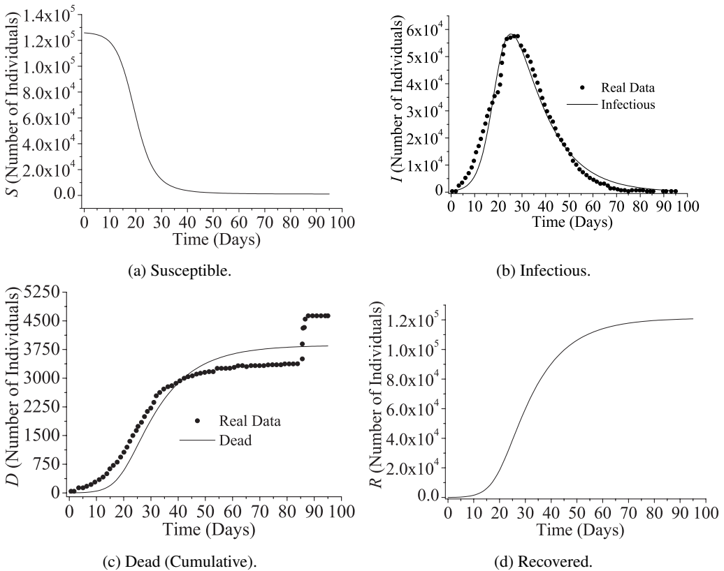
Figure 2: Simulated and reported profiles considering the best estimated parameters.
