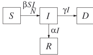
Figure 1: Compartments in the SIRD model [1, 3].
