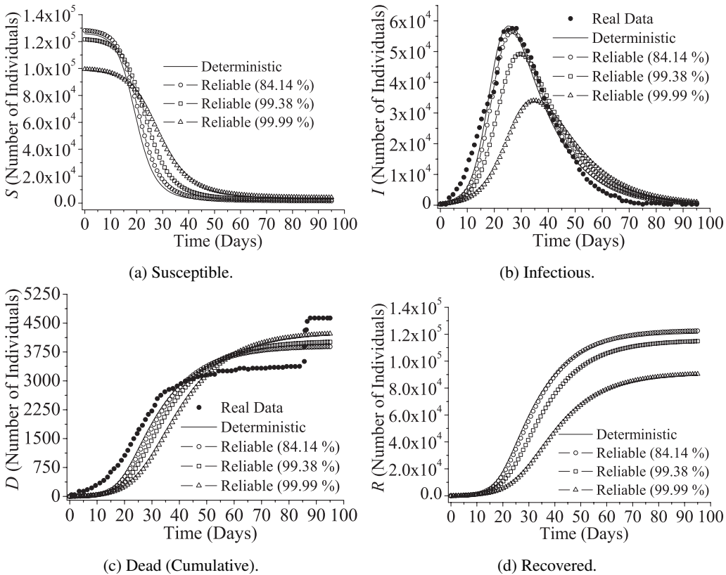
Figure 4: Simulated and reported profiles considering the best estimated parameters by using \Omega = \{1, 2.5, 5\} , cov = 0.05 and Normal distribution.
