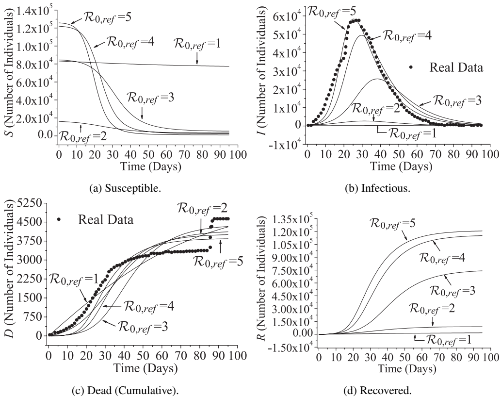
Figure 3: Simulated and reported profiles considering different values for the parameter \mathcal{R}_{0,ref} .
