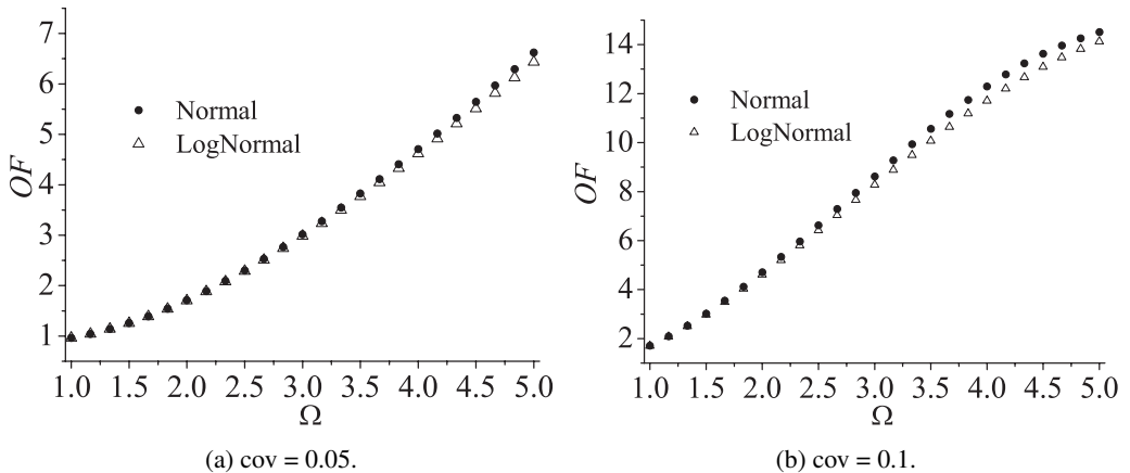
Figure 5: Influence of the type of distribution and the coefficient of variation considering the solution obtained by IRA.
