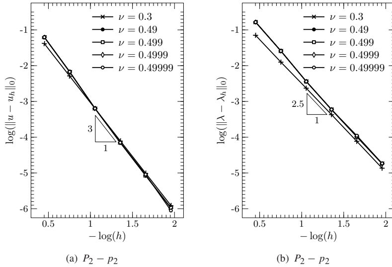
Figure 2: h -convergence study for \mathbf{u}_h and \lambda_h of primal SHDG approximations with \nu = 0.3, 0.49, 0.499, 0.4999, 0.49999 .
