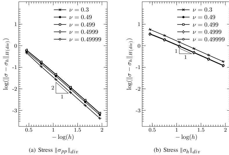
Figure 6: h-Convergence for \sigma_{pp} and \sigma_h approximations in H(\text{div}) norm using k + 1 = 3 and \nu = 0.3, 0.49, 0.499, 0.4999, 0.49999 .
