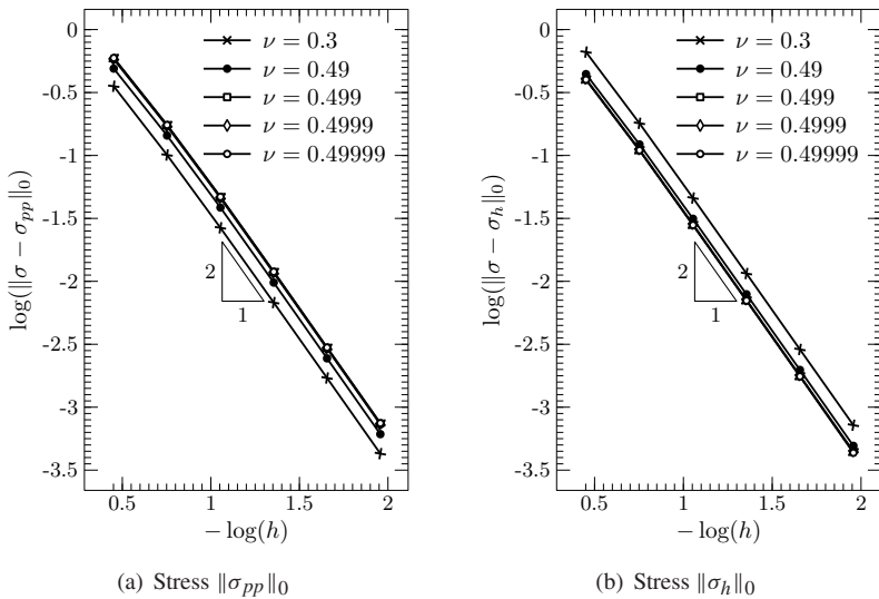
Figure 5: h -Convergence for \sigma_{pp} and \sigma_h approximations in L_2 norm using k + 1 = 3 and \nu = 0.3, 0.49, 0.499, 0.4999, 0.49999 .
